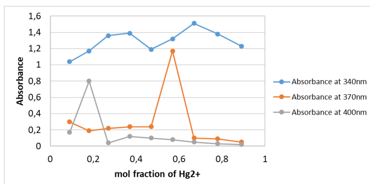
Figure 3. Absorbance versus mol fraction of \text{Hg}^{2+} .
