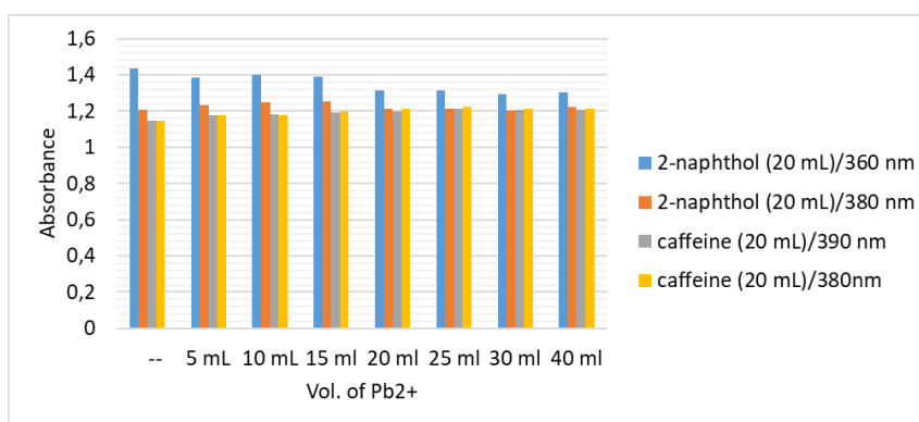
Figure 4. Absorbance versus Vol. of Pb 2+ .
