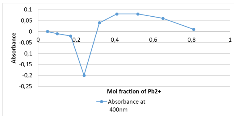
Figure 2. Absorbance versus mol fraction of \text{Pb}^{2+} .
