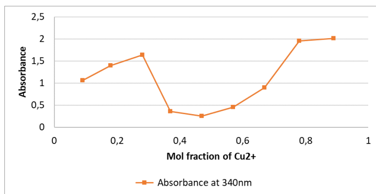
Figure 1. Absorbance versus mol fraction of \text{Cu}^{2+} .
