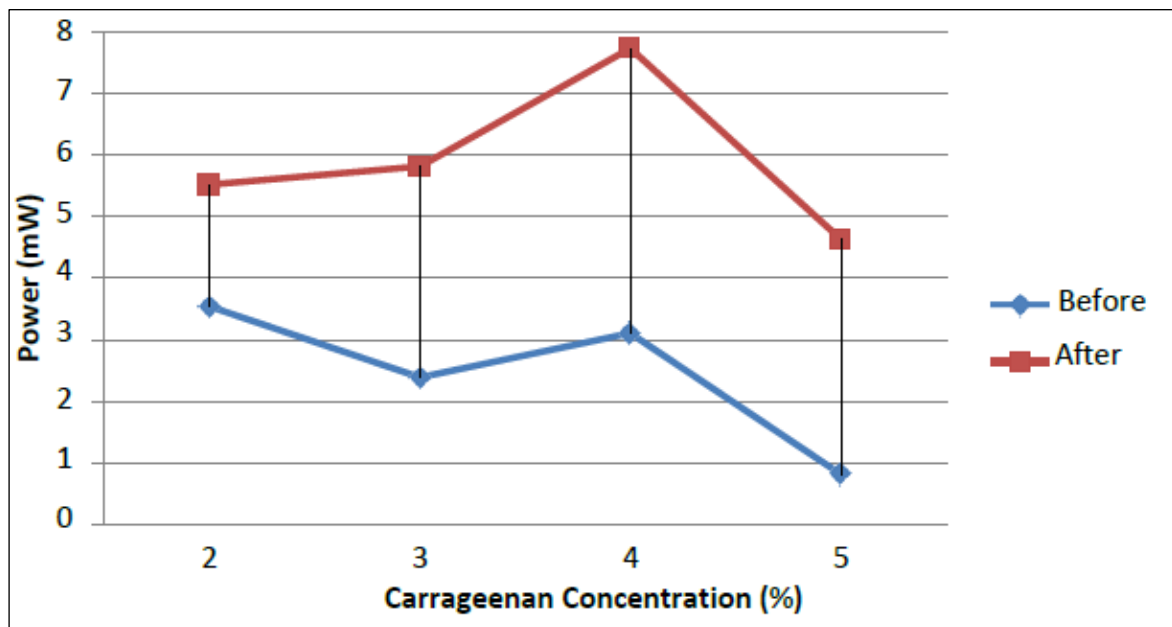
Figure 6. Power comparison curve before and after recharging in the second experiment.
